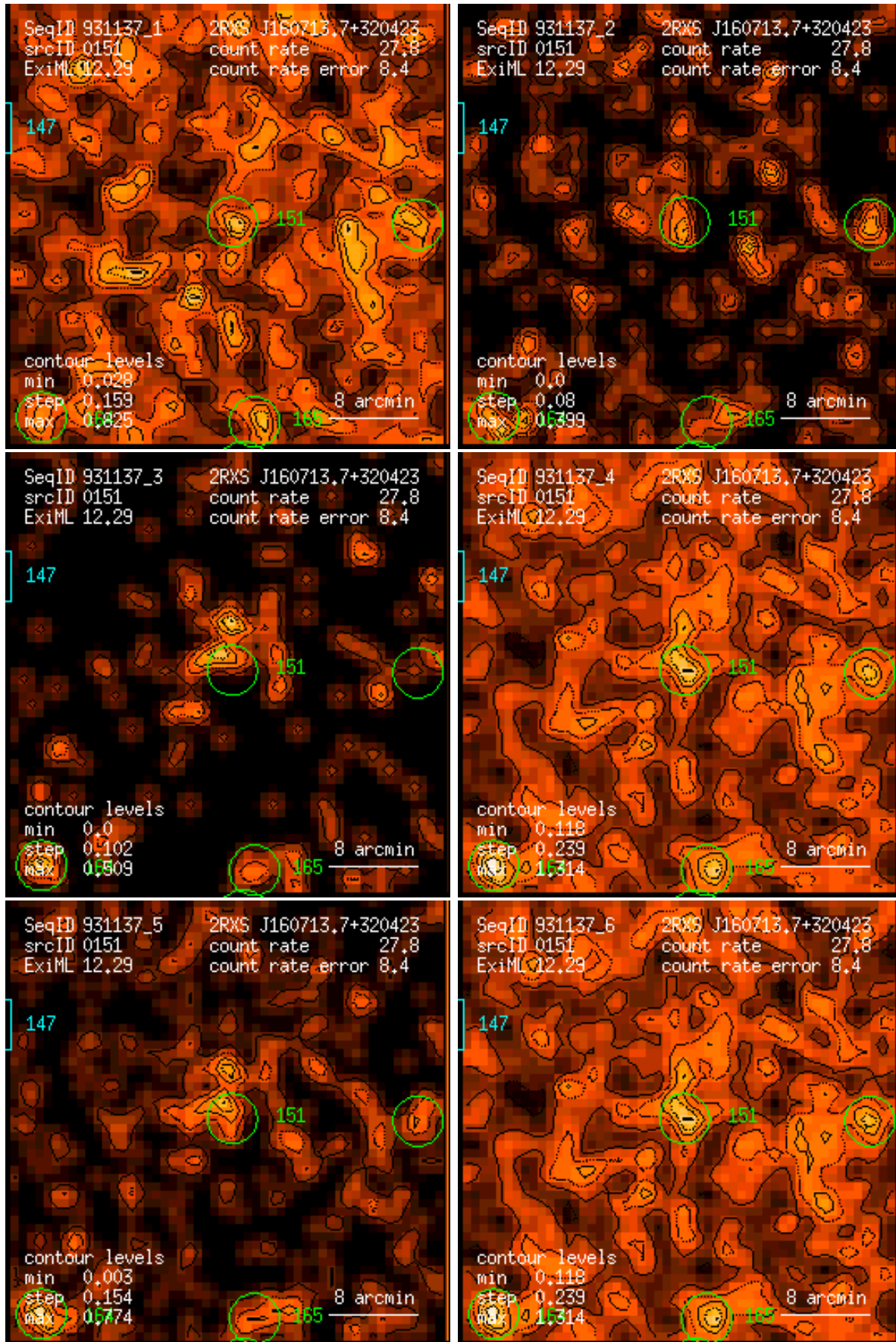
Figure 151: RASS 931137: detection 0151: band rate images, Gaussian filter: (1) PSPC channels 11 – 41, (2) 52 – 90, (3) 91 – 201, (4) 11 – 235, (5) 52 – 201, (6) 11 – 201. Broad band rates in counts/ks. Band rate contour levels in counts/ks/arcmin 2 .
