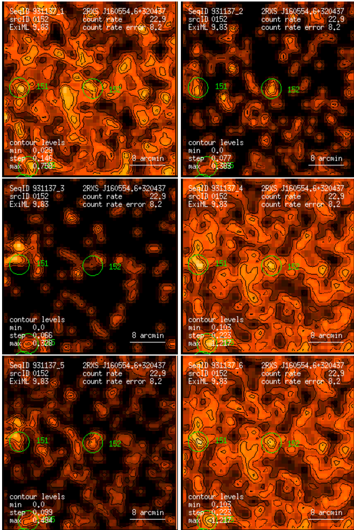
Figure 152: RASS 931137: detection 0152: band rate images, Gaussian filter: (1) PSPC channels 11 – 41, (2) 52 – 90, (3) 91 – 201, (4) 11 – 235, (5) 52 – 201, (6) 11 – 201. Broad band rates in counts/ks. Band rate contour levels in counts/ks/arcmin 2 .
