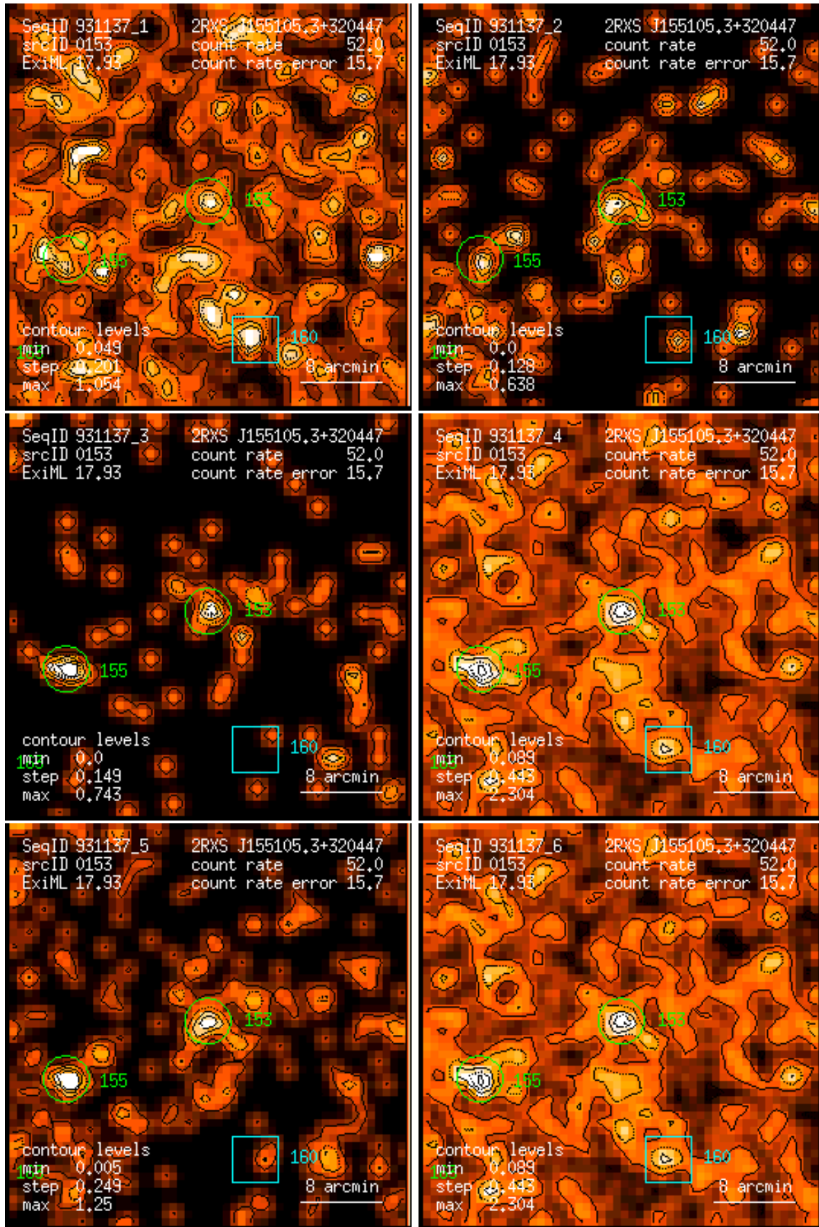
Figure 153: RASS 931137: detection 0153: band rate images, Gaussian filter: (1) PSPC channels 11 – 41, (2) 52 – 90, (3) 91 – 201, (4) 11 – 235, (5) 52 – 201, (6) 11 – 201. Broad band rates in counts/ks. Band rate contour levels in counts/ks/arcmin 2 .
