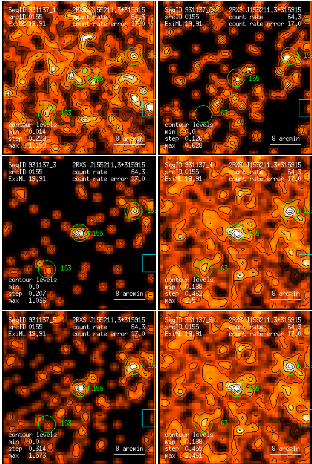
Figure 155: RASS 931137: detection 0155: band rate images, Gaussian filter: (1) PSPC channels 11 – 41, (2) 52 – 90, (3) 91 – 201, (4) 11 – 235, (5) 52 – 201, (6) 11 – 201. Broad band rates in counts/ks. Band rate contour levels in counts/ks/arcmin 2 .
