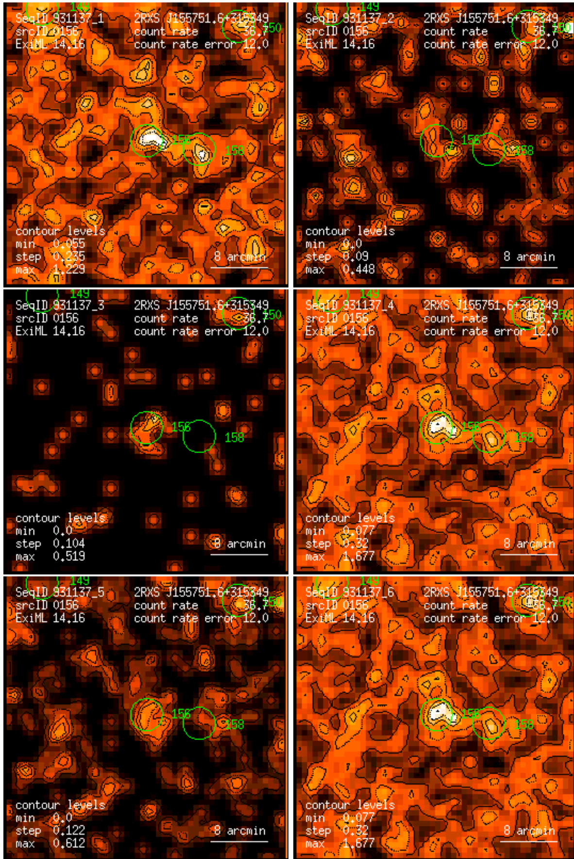
Figure 156: RASS 931137: detection 0156: band rate images, Gaussian filter: (1) PSPC channels 11 – 41, (2) 52 – 90, (3) 91 – 201, (4) 11 – 235, (5) 52 – 201, (6) 11 – 201. Broad band rates in counts/ks. Band rate contour levels in counts/ks/arcmin 2 .
