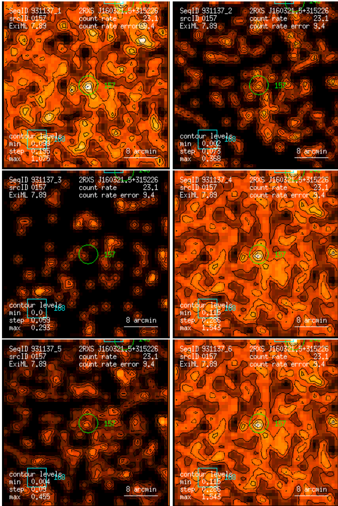
Figure 157: RASS 931137: detection 0157: band rate images, Gaussian filter: (1) PSPC channels 11 – 41, (2) 52 – 90, (3) 91 – 201, (4) 11 – 235, (5) 52 – 201, (6) 11 – 201. Broad band rates in counts/ks. Band rate contour levels in counts/ks/arcmin 2 .
