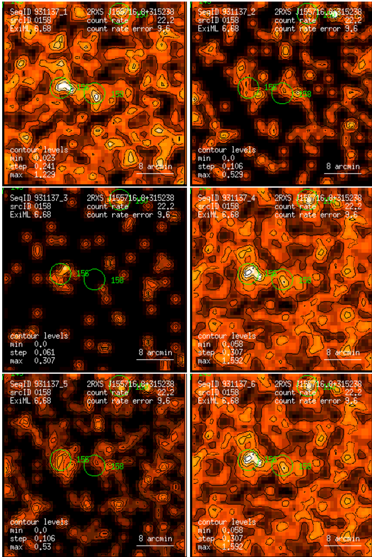
Figure 158: RASS 931137: detection 0158: band rate images, Gaussian filter: (1) PSPC channels 11 – 41, (2) 52 – 90, (3) 91 – 201, (4) 11 – 235, (5) 52 – 201, (6) 11 – 201. Broad band rates in counts/ks. Band rate contour levels in counts/ks/arcmin 2 .
