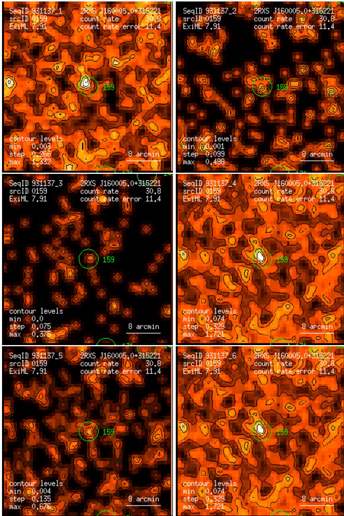
Figure 159: RASS 931137: detection 0159: band rate images, Gaussian filter: (1) PSPC channels 11 – 41, (2) 52 – 90, (3) 91 – 201, (4) 11 – 235, (5) 52 – 201, (6) 11 – 201. Broad band rates in counts/ks. Band rate contour levels in counts/ks/arcmin 2 .
