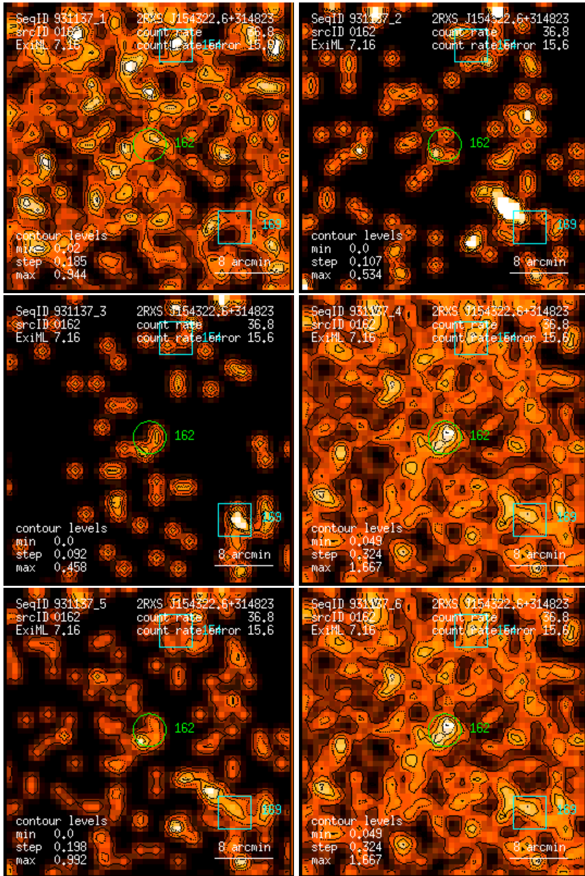
Figure 162: RASS 931137: detection 0162: band rate images, Gaussian filter: (1) PSPC channels 11 – 41, (2) 52 – 90, (3) 91 – 201, (4) 11 – 235, (5) 52 – 201, (6) 11 – 201. Broad band rates in counts/ks. Band rate contour levels in counts/ks/arcmin 2 .
