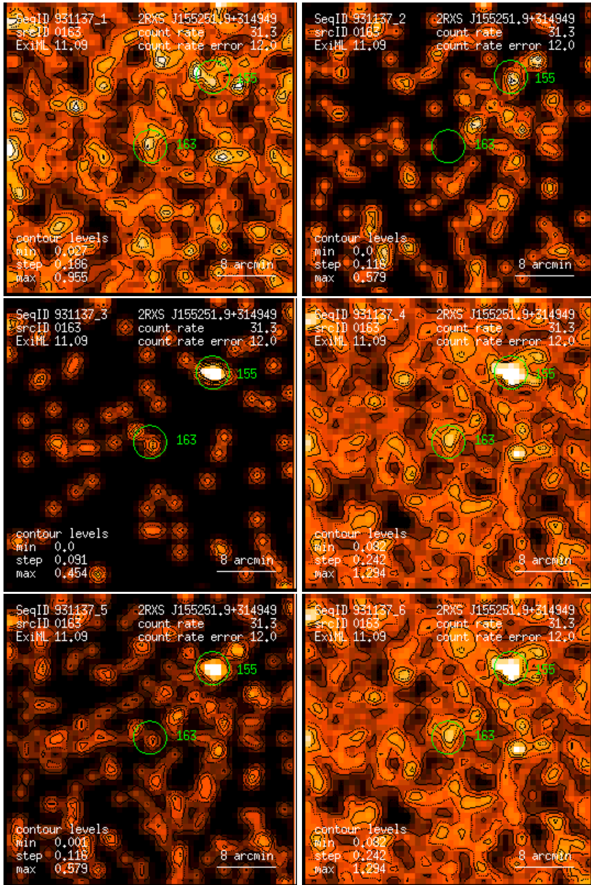
Figure 163: RASS 931137: detection 0163: band rate images, Gaussian filter: (1) PSPC channels 11 – 41, (2) 52 – 90, (3) 91 – 201, (4) 11 – 235, (5) 52 – 201, (6) 11 – 201. Broad band rates in counts/ks. Band rate contour levels in counts/ks/arcmin 2 .
