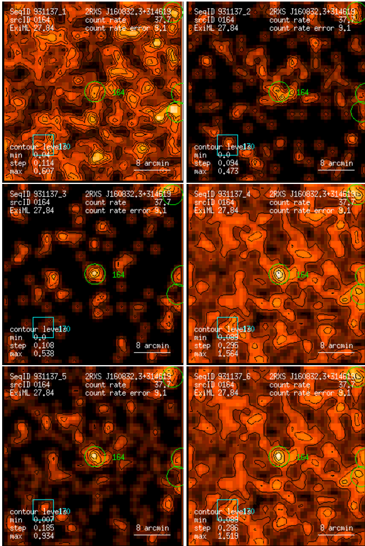
Figure 164: RASS 931137: detection 0164: band rate images, Gaussian filter: (1) PSPC channels 11 – 41, (2) 52 – 90, (3) 91 – 201, (4) 11 – 235, (5) 52 – 201, (6) 11 – 201. Broad band rates in counts/ks. Band rate contour levels in counts/ks/arcmin 2 .
