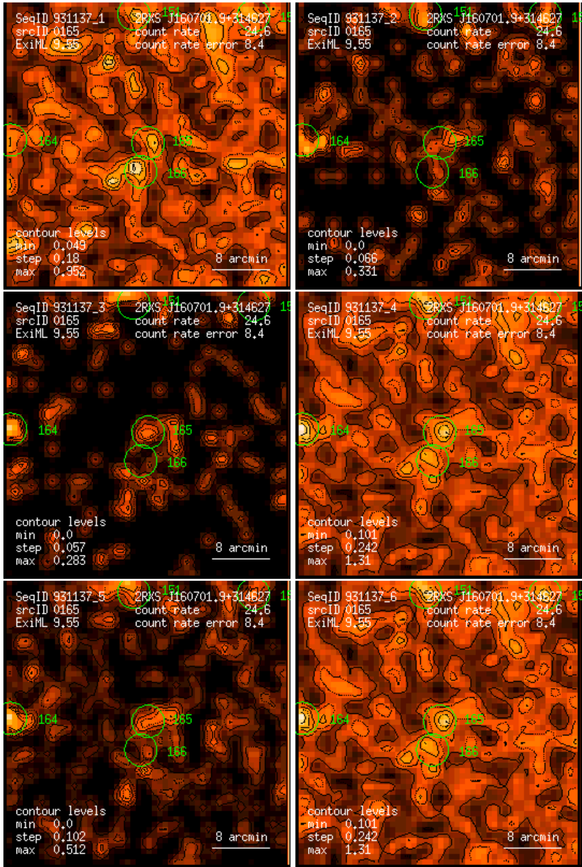
Figure 165: RASS 931137: detection 0165: band rate images, Gaussian filter: (1) PSPC channels 11 – 41, (2) 52 – 90, (3) 91 – 201, (4) 11 – 235, (5) 52 – 201, (6) 11 – 201. Broad band rates in counts/ks. Band rate contour levels in counts/ks/arcmin 2 .
