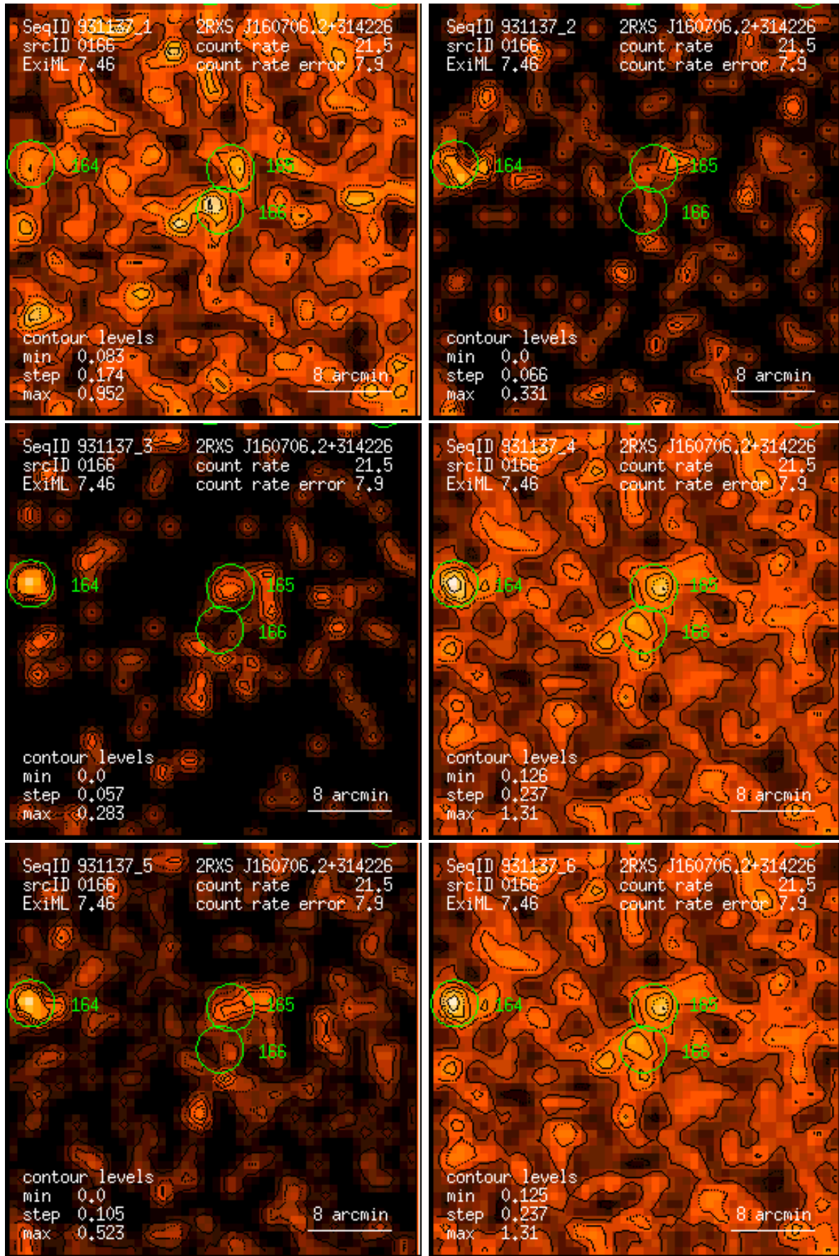
Figure 166: RASS 931137: detection 0166: band rate images, Gaussian filter: (1) PSPC channels 11 – 41, (2) 52 – 90, (3) 91 – 201, (4) 11 – 235, (5) 52 – 201, (6) 11 – 201. Broad band rates in counts/ks. Band rate contour levels in counts/ks/arcmin 2 .
