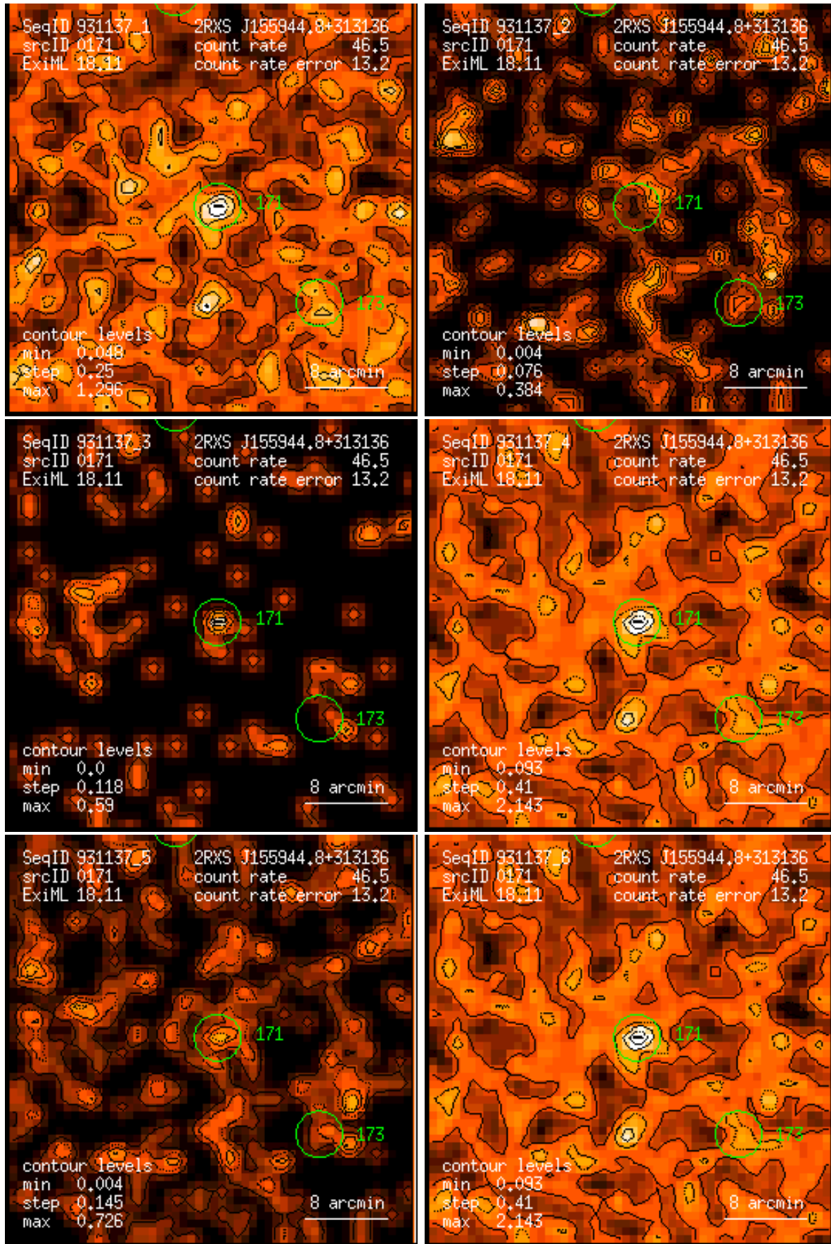
Figure 171: RASS 931137: detection 0171: band rate images, Gaussian filter: (1) PSPC channels 11 – 41, (2) 52 – 90, (3) 91 – 201, (4) 11 – 235, (5) 52 – 201, (6) 11 – 201. Broad band rates in counts/ks. Band rate contour levels in counts/ks/arcmin 2 .
