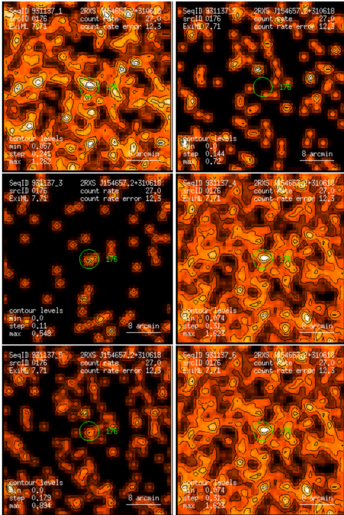
Figure 176: RASS 931137: detection 0176: band rate images, Gaussian filter: (1) PSPC channels 11 – 41, (2) 52 – 90, (3) 91 – 201, (4) 11 – 235, (5) 52 – 201, (6) 11 – 201. Broad band rates in counts/ks. Band rate contour levels in counts/ks/arcmin 2 .
