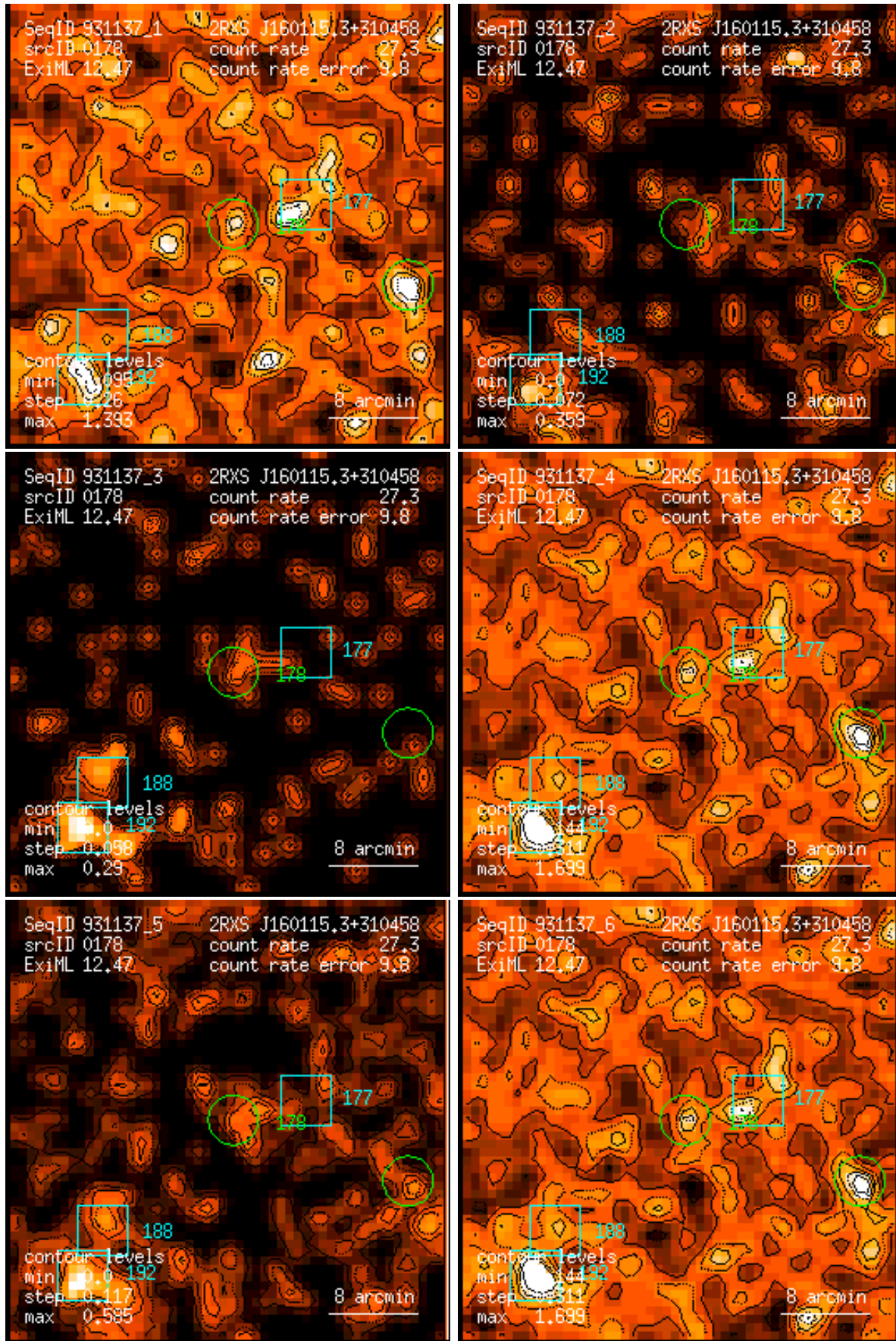
Figure 178: RASS 931137: detection 0178: band rate images, Gaussian filter: (1) PSPC channels 11 – 41, (2) 52 – 90, (3) 91 – 201, (4) 11 – 235, (5) 52 – 201, (6) 11 – 201. Broad band rates in counts/ks. Band rate contour levels in counts/ks/arcmin 2 .
