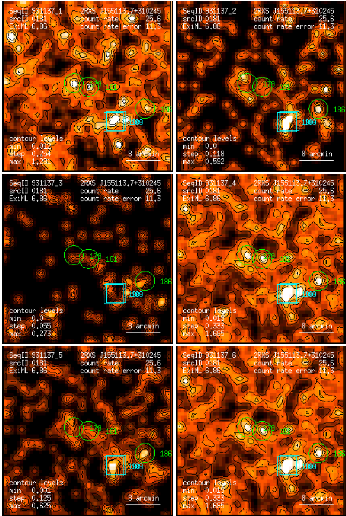
Figure 181: RASS 931137: detection 0181: band rate images, Gaussian filter: (1) PSPC channels 11 – 41, (2) 52 – 90, (3) 91 – 201, (4) 11 – 235, (5) 52 – 201, (6) 11 – 201. Broad band rates in counts/ks. Band rate contour levels in counts/ks/arcmin 2 .
