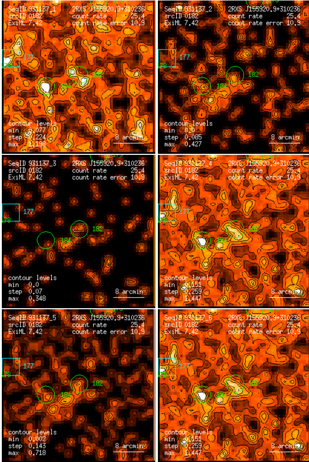
Figure 182: RASS 931137: detection 0182: band rate images, Gaussian filter: (1) PSPC channels 11 – 41, (2) 52 – 90, (3) 91 – 201, (4) 11 – 235, (5) 52 – 201, (6) 11 – 201. Broad band rates in counts/ks. Band rate contour levels in counts/ks/arcmin 2 .
