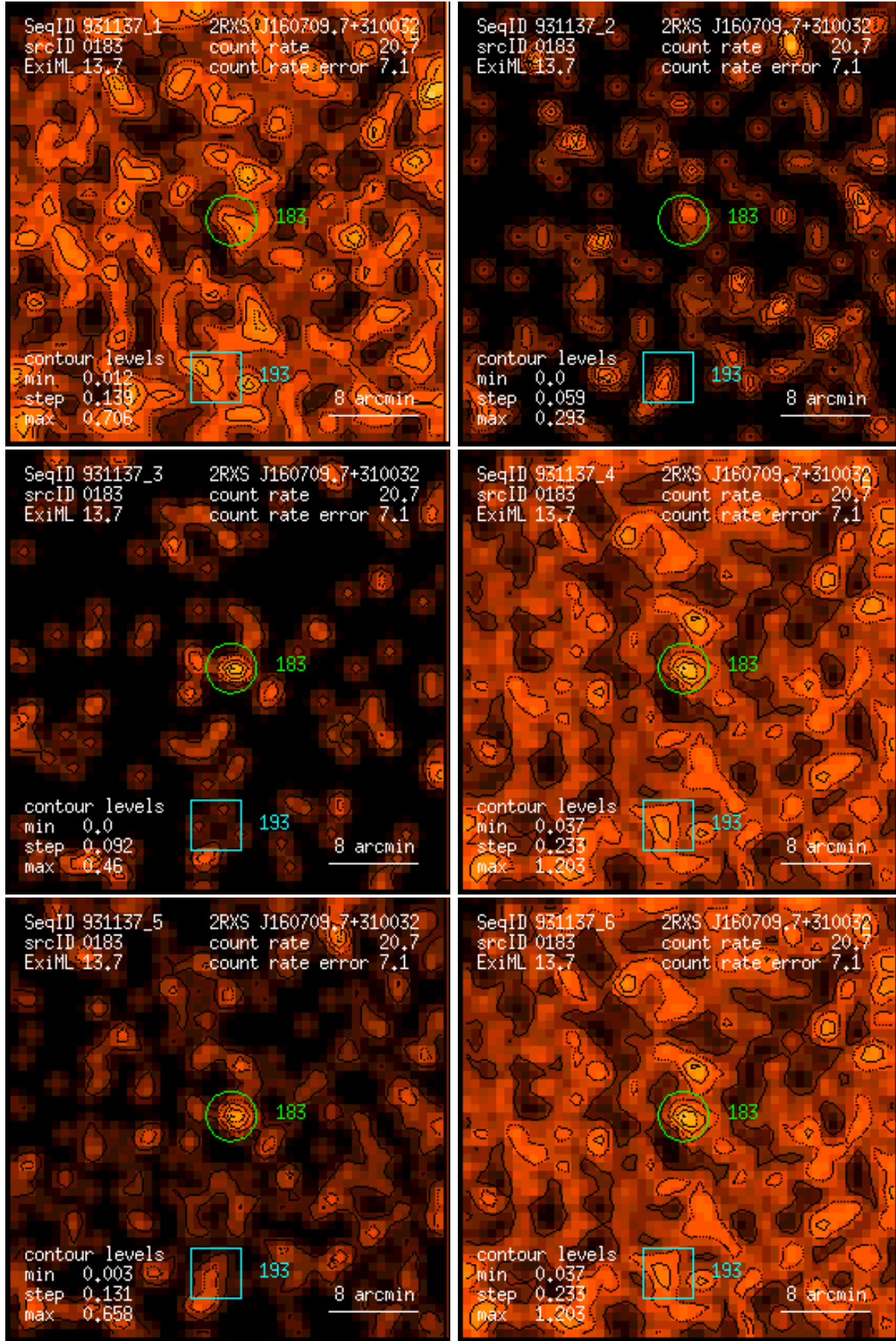
Figure 183: RASS 931137: detection 0183: band rate images, Gaussian filter: (1) PSPC channels 11 – 41, (2) 52 – 90, (3) 91 – 201, (4) 11 – 235, (5) 52 – 201, (6) 11 – 201. Broad band rates in counts/ks. Band rate contour levels in counts/ks/arcmin 2 .
