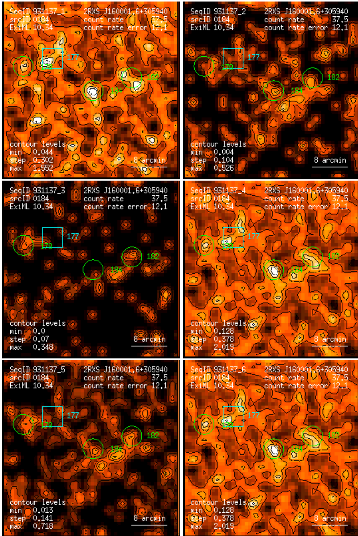
Figure 184: RASS 931137: detection 0184: band rate images, Gaussian filter: (1) PSPC channels 11 – 41, (2) 52 – 90, (3) 91 – 201, (4) 11 – 235, (5) 52 – 201, (6) 11 – 201. Broad band rates in counts/ks. Band rate contour levels in counts/ks/arcmin 2 .
