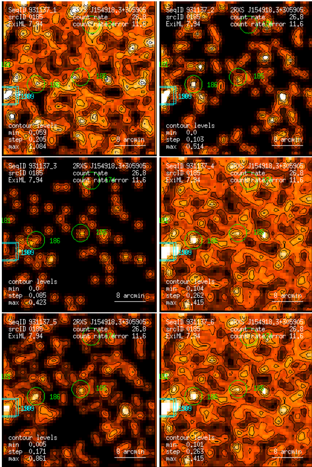
Figure 185: RASS 931137: detection 0185: band rate images, Gaussian filter: (1) PSPC channels 11 – 41, (2) 52 – 90, (3) 91 – 201, (4) 11 – 235, (5) 52 – 201, (6) 11 – 201. Broad band rates in counts/ks. Band rate contour levels in counts/ks/arcmin 2 .
