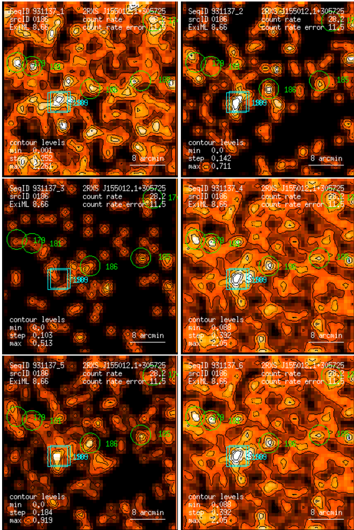
Figure 186: RASS 931137: detection 0186: band rate images, Gaussian filter: (1) PSPC channels 11 – 41, (2) 52 – 90, (3) 91 – 201, (4) 11 – 235, (5) 52 – 201, (6) 11 – 201. Broad band rates in counts/ks. Band rate contour levels in counts/ks/arcmin 2 .
