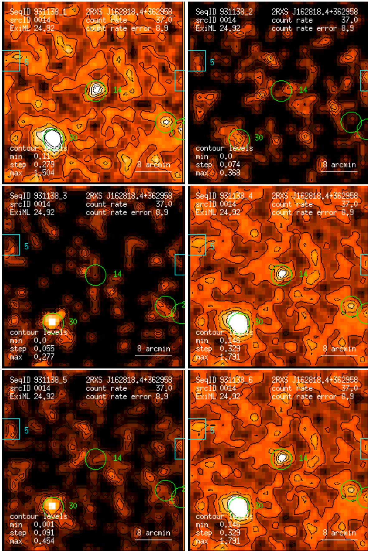
Figure 14: RASS 931138: detection 0014: band rate images, Gaussian filter: (1) PSPC channels 11 – 41, (2) 52 – 90, (3) 91 – 201, (4) 11 – 235, (5) 52 – 201, (6) 11 – 201. Broad band rates in counts/ks. Band rate contour levels in counts/ks/arcmin 2 .
