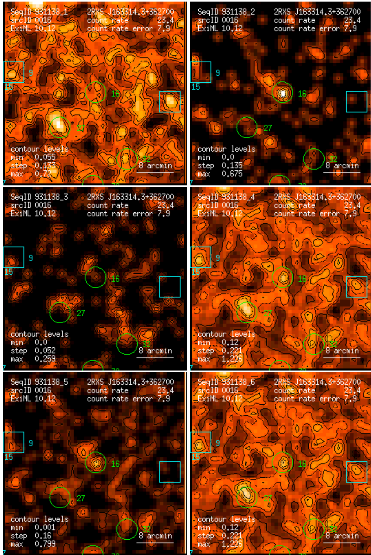
Figure 16: RASS 931138: detection 0016: band rate images, Gaussian filter: (1) PSPC channels 11 – 41, (2) 52 – 90, (3) 91 – 201, (4) 11 – 235, (5) 52 – 201, (6) 11 – 201. Broad band rates in counts/ks. Band rate contour levels in counts/ks/arcmin 2 .
