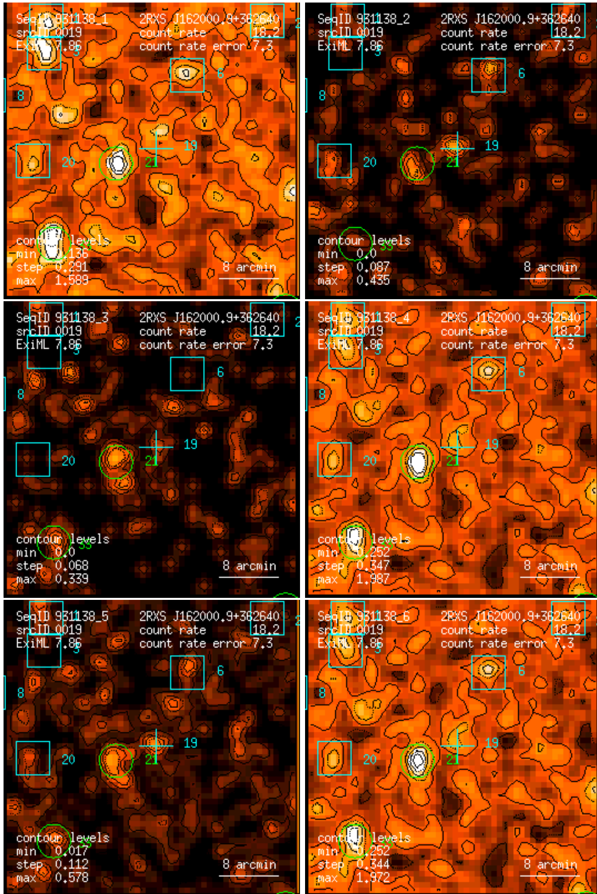
Figure 19: RASS 931138: detection 0019: band rate images, Gaussian filter: (1) PSPC channels 11 – 41, (2) 52 – 90, (3) 91 – 201, (4) 11 – 235, (5) 52 – 201, (6) 11 – 201. Broad band rates in counts/ks. Band rate contour levels in counts/ks/arcmin 2 .
