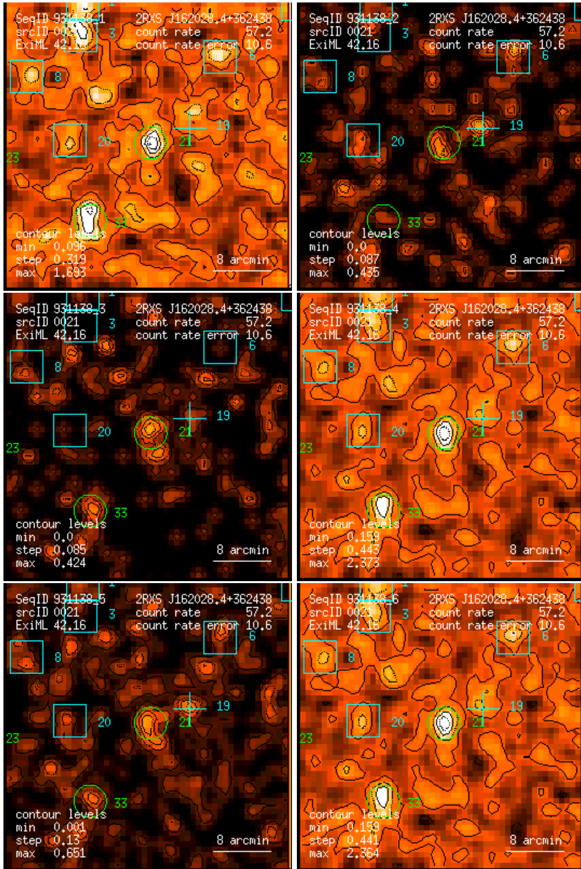
Figure 21: RASS 931138: detection 0021: band rate images, Gaussian filter: (1) PSPC channels 11 – 41, (2) 52 – 90, (3) 91 – 201, (4) 11 – 235, (5) 52 – 201, (6) 11 – 201. Broad band rates in counts/ks. Band rate contour levels in counts/ks/arcmin 2 .
