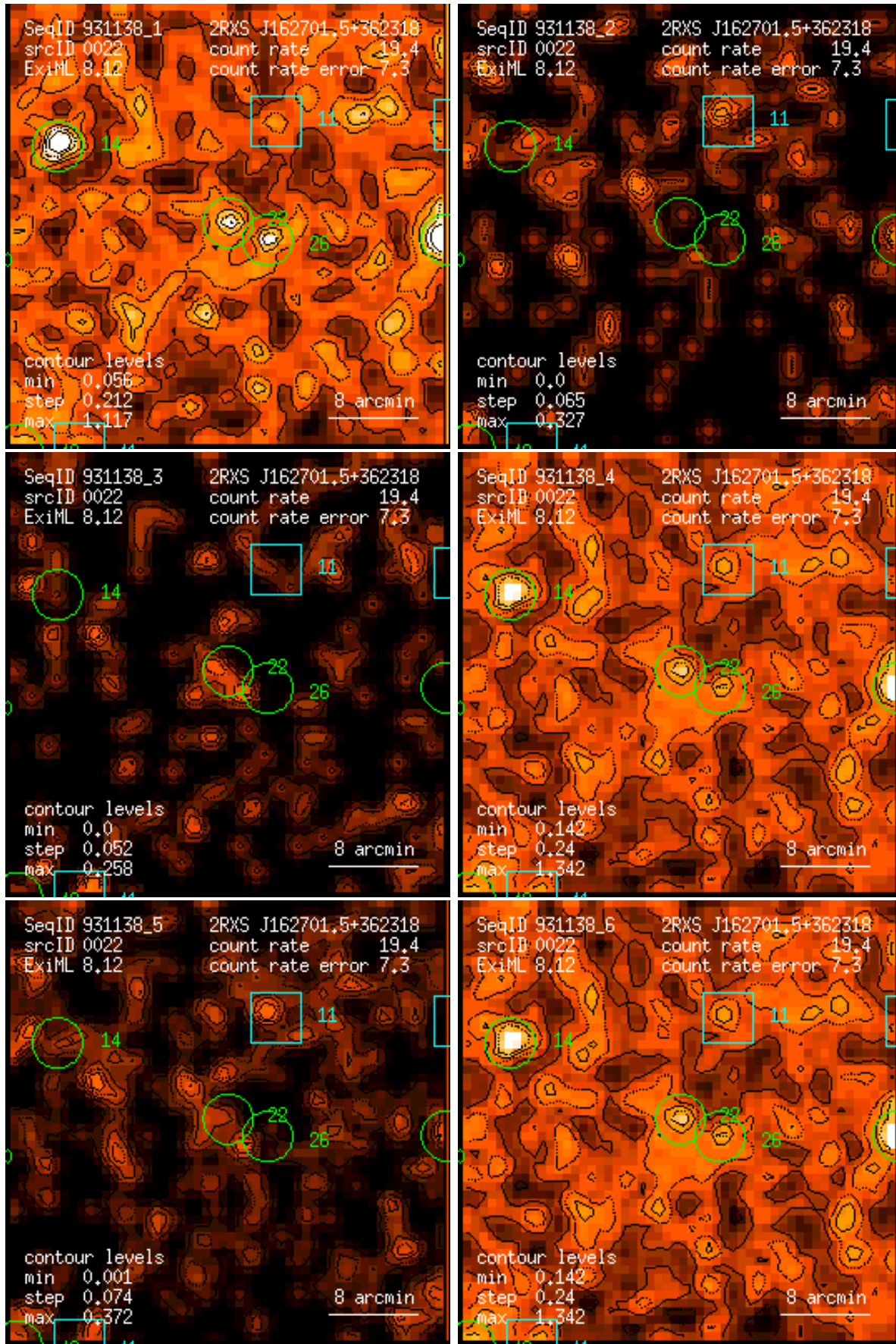
Figure 22: RASS 931138: detection 0022: band rate images, Gaussian filter: (1) PSPC channels 11 – 41, (2) 52 – 90, (3) 91 – 201, (4) 11 – 235, (5) 52 – 201, (6) 11 – 201. Broad band rates in counts/ks. Band rate contour levels in counts/ks/arcmin 2 .
