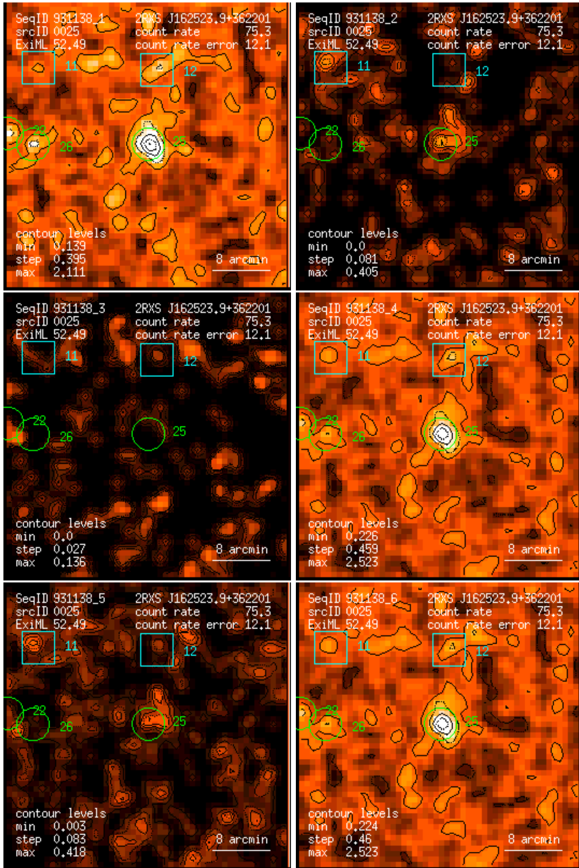
Figure 25: RASS 931138: detection 0025: band rate images, Gaussian filter: (1) PSPC channels 11 – 41, (2) 52 – 90, (3) 91 – 201, (4) 11 – 235, (5) 52 – 201, (6) 11 – 201. Broad band rates in counts/ks. Band rate contour levels in counts/ks/arcmin 2 .
