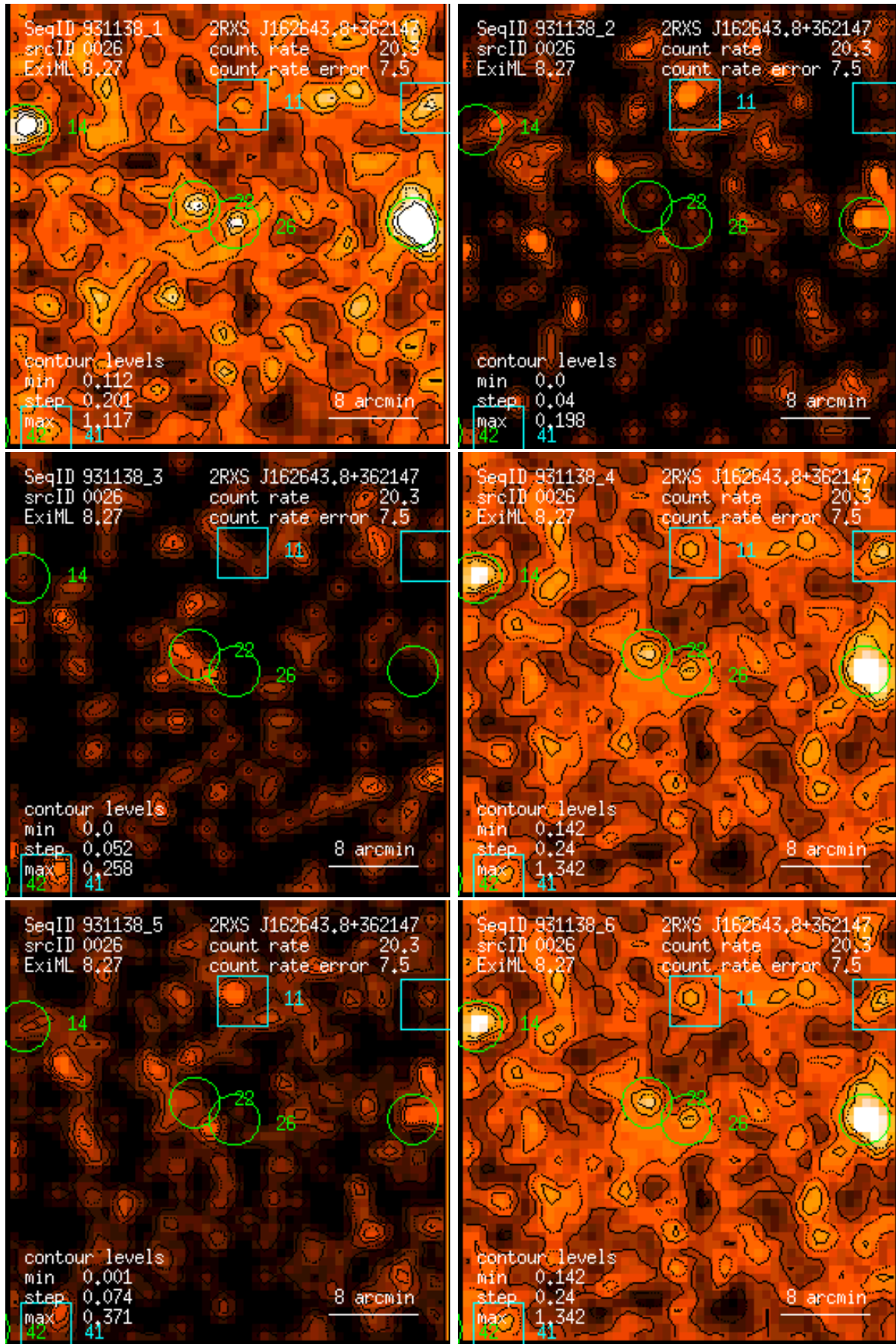
Figure 26: RASS 931138: detection 0026: band rate images, Gaussian filter: (1) PSPC channels 11 – 41, (2) 52 – 90, (3) 91 – 201, (4) 11 – 235, (5) 52 – 201, (6) 11 – 201. Broad band rates in counts/ks. Band rate contour levels in counts/ks/arcmin 2 .
