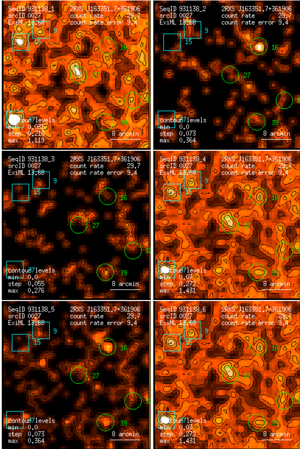
Figure 27: RASS 931138: detection 0027: band rate images, Gaussian filter: (1) PSPC channels 11 – 41, (2) 52 – 90, (3) 91 – 201, (4) 11 – 235, (5) 52 – 201, (6) 11 – 201. Broad band rates in counts/ks. Band rate contour levels in counts/ks/arcmin 2 .
