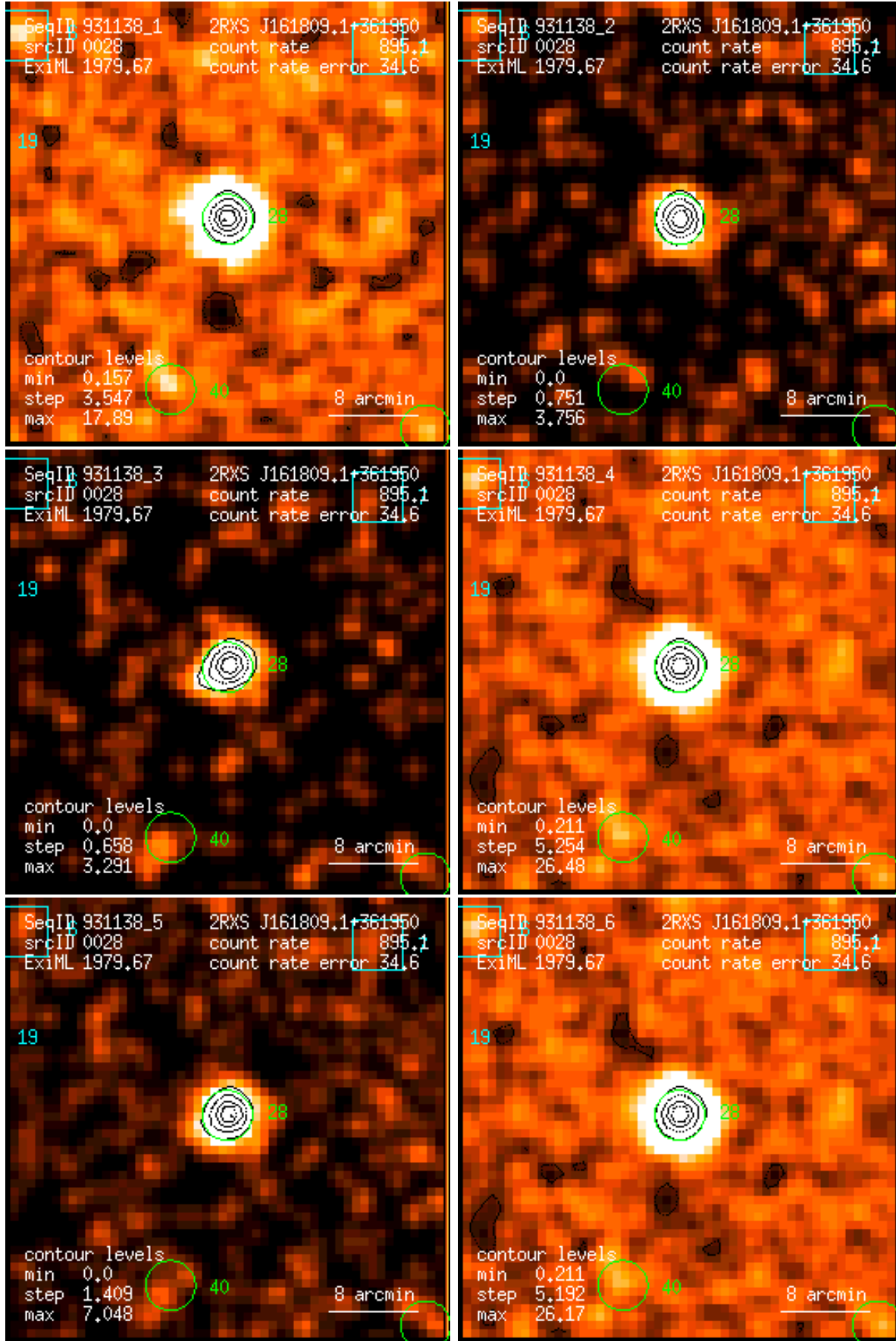
Figure 28: RASS 931138: detection 0028: band rate images, Gaussian filter: (1) PSPC channels 11 – 41, (2) 52 – 90, (3) 91 – 201, (4) 11 – 235, (5) 52 – 201, (6) 11 – 201. Broad band rates in counts/ks. Band rate contour levels in counts/ks/arcmin 2 .
