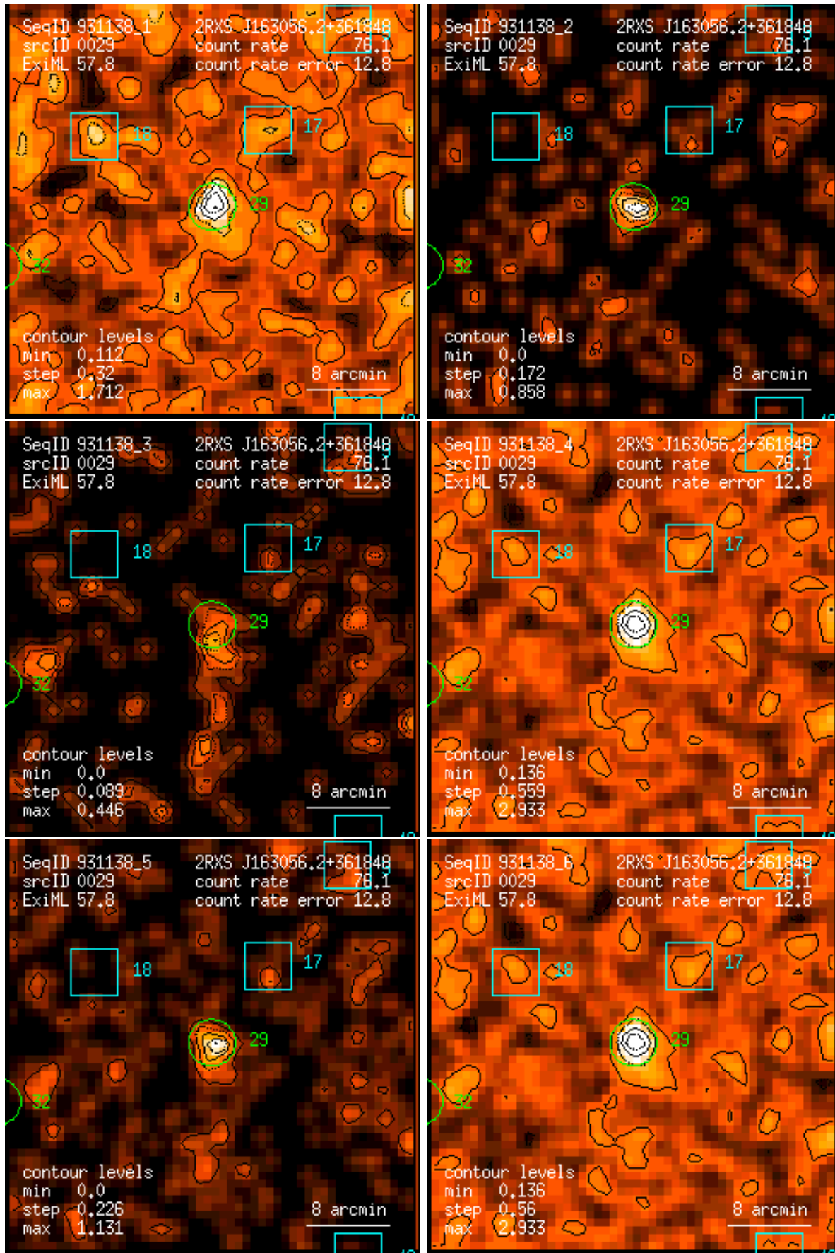
Figure 29: RASS 931138: detection 0029: band rate images, Gaussian filter: (1) PSPC channels 11 – 41, (2) 52 – 90, (3) 91 – 201, (4) 11 – 235, (5) 52 – 201, (6) 11 – 201. Broad band rates in counts/ks. Band rate contour levels in counts/ks/arcmin 2 .
