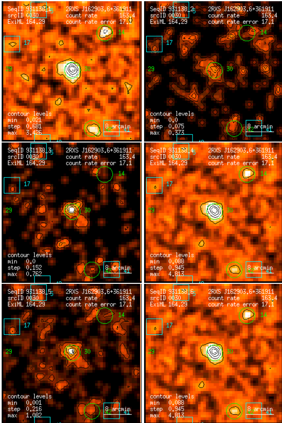
Figure 30: RASS 931138: detection 0030: band rate images, Gaussian filter: (1) PSPC channels 11 – 41, (2) 52 – 90, (3) 91 – 201, (4) 11 – 235, (5) 52 – 201, (6) 11 – 201. Broad band rates in counts/ks. Band rate contour levels in counts/ks/arcmin 2 .
