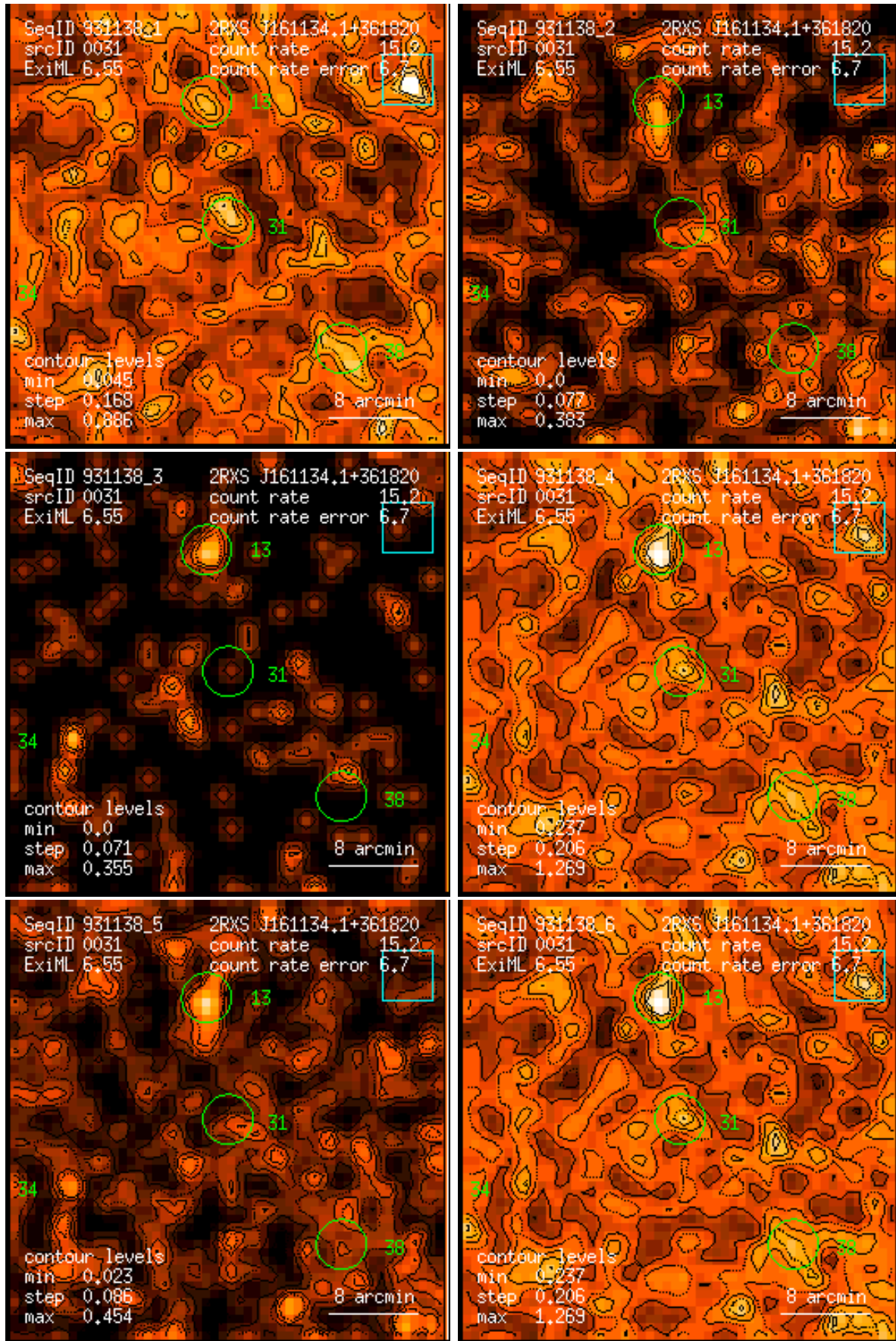
Figure 31: RASS 931138: detection 0031: band rate images, Gaussian filter: (1) PSPC channels 11 – 41, (2) 52 – 90, (3) 91 – 201, (4) 11 – 235, (5) 52 – 201, (6) 11 – 201. Broad band rates in counts/ks. Band rate contour levels in counts/ks/arcmin 2 .
