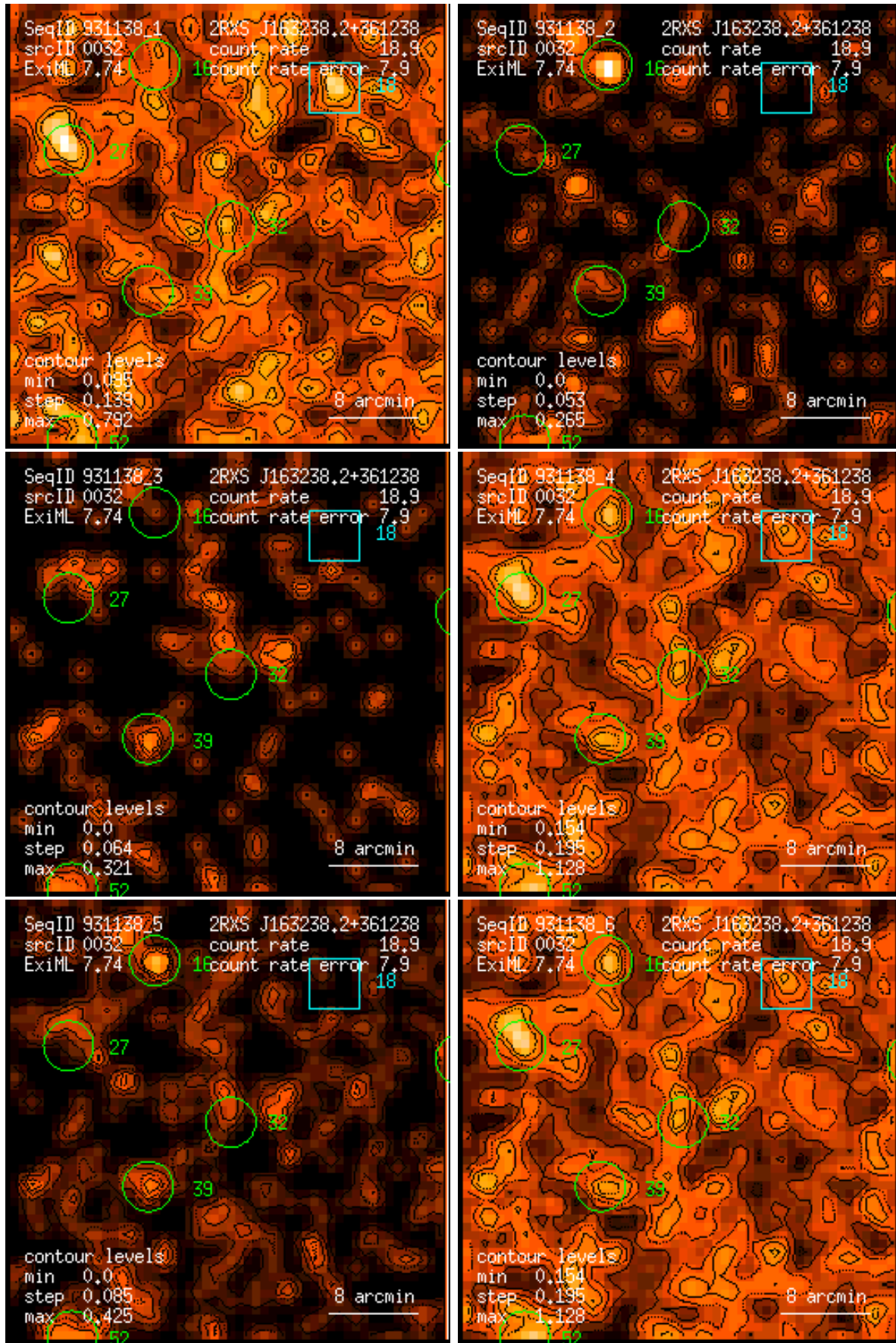
Figure 32: RASS 931138: detection 0032: band rate images, Gaussian filter: (1) PSPC channels 11 – 41, (2) 52 – 90, (3) 91 – 201, (4) 11 – 235, (5) 52 – 201, (6) 11 – 201. Broad band rates in counts/ks. Band rate contour levels in counts/ks/arcmin 2 .
