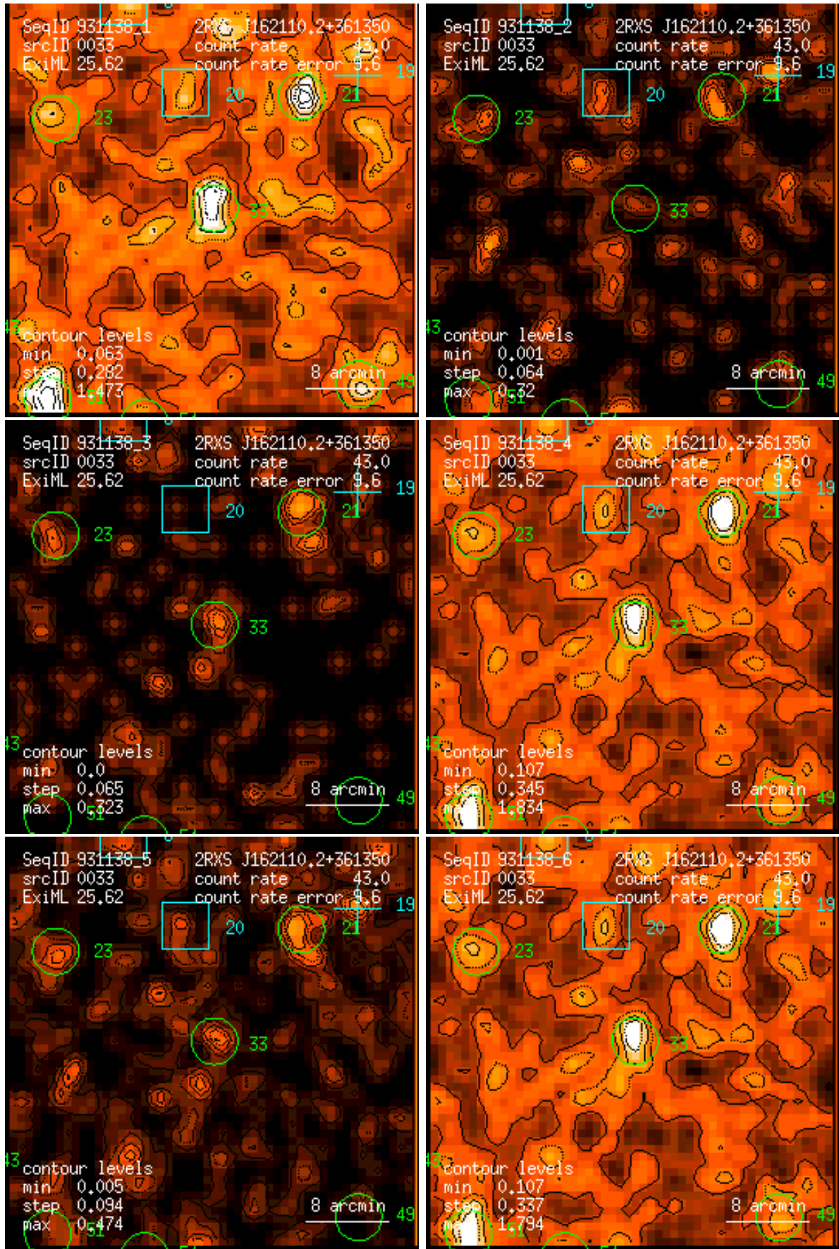
Figure 33: RASS 931138: detection 0033: band rate images, Gaussian filter: (1) PSPC channels 11 – 41, (2) 52 – 90, (3) 91 – 201, (4) 11 – 235, (5) 52 – 201, (6) 11 – 201. Broad band rates in counts/ks. Band rate contour levels in counts/ks/arcmin 2 .
