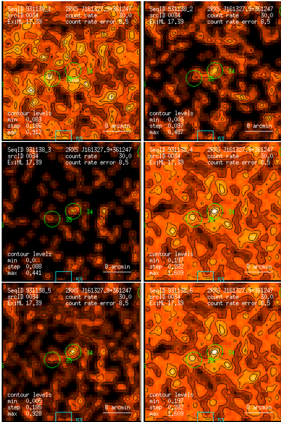
Figure 34: RASS 931138: detection 0034: band rate images, Gaussian filter: (1) PSPC channels 11 – 41, (2) 52 – 90, (3) 91 – 201, (4) 11 – 235, (5) 52 – 201, (6) 11 – 201. Broad band rates in counts/ks. Band rate contour levels in counts/ks/arcmin 2 .
