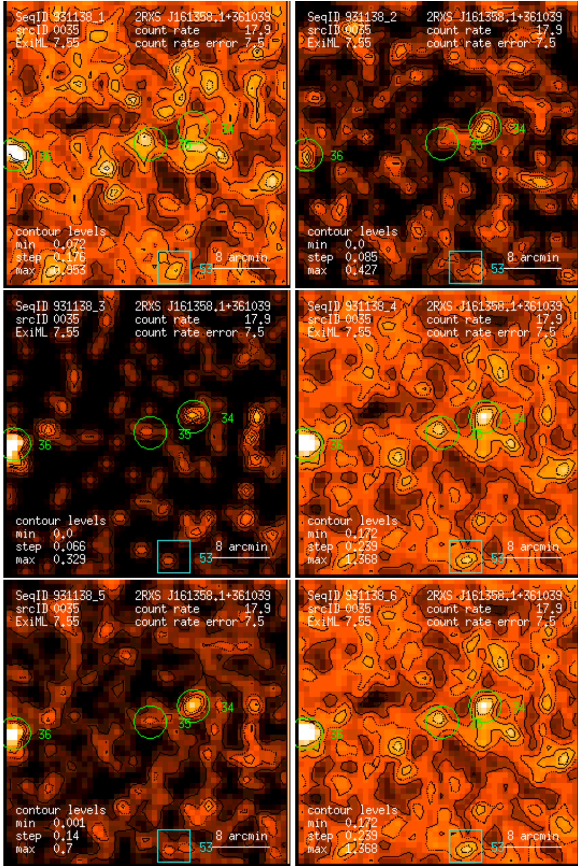
Figure 35: RASS 931138: detection 0035: band rate images, Gaussian filter: (1) PSPC channels 11 – 41, (2) 52 – 90, (3) 91 – 201, (4) 11 – 235, (5) 52 – 201, (6) 11 – 201. Broad band rates in counts/ks. Band rate contour levels in counts/ks/arcmin 2 .
