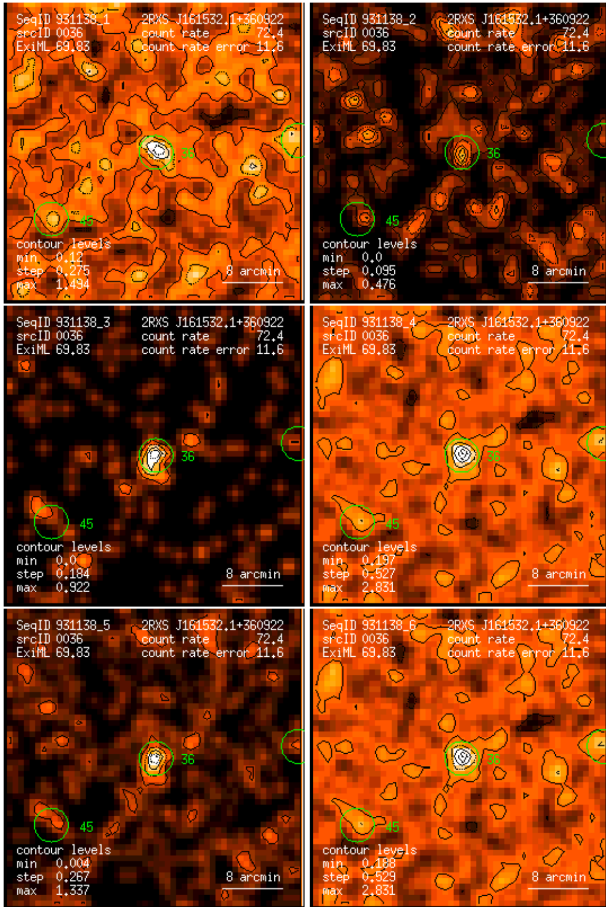
Figure 36: RASS 931138: detection 0036: band rate images, Gaussian filter: (1) PSPC channels 11 – 41, (2) 52 – 90, (3) 91 – 201, (4) 11 – 235, (5) 52 – 201, (6) 11 – 201. Broad band rates in counts/ks. Band rate contour levels in counts/ks/arcmin 2 .
