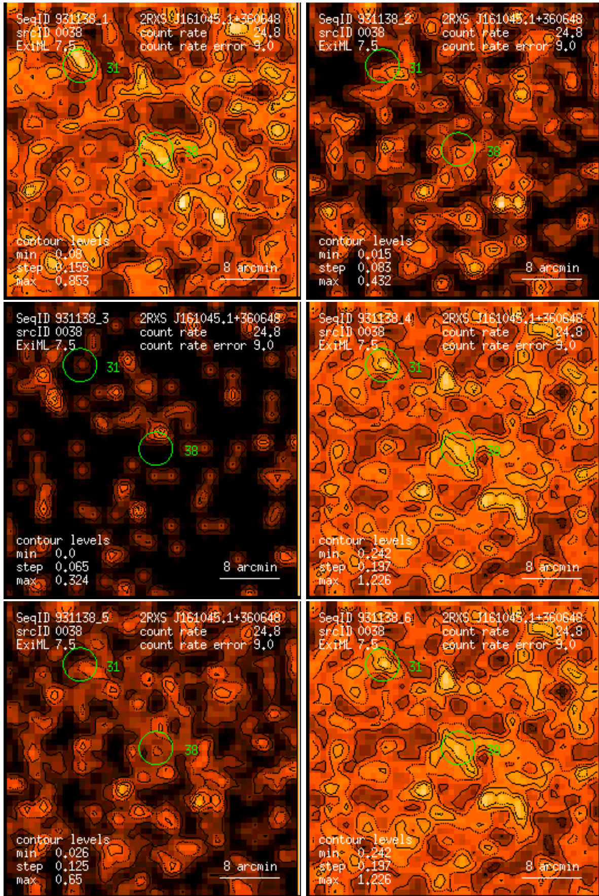
Figure 38: RASS 931138: detection 0038: band rate images, Gaussian filter: (1) PSPC channels 11 – 41, (2) 52 – 90, (3) 91 – 201, (4) 11 – 235, (5) 52 – 201, (6) 11 – 201. Broad band rates in counts/ks. Band rate contour levels in counts/ks/arcmin 2 .
