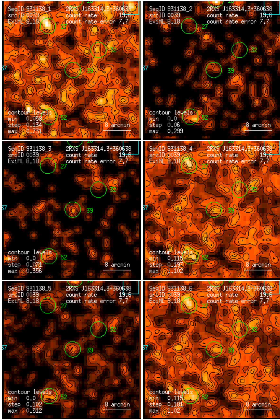
Figure 39: RASS 931138: detection 0039: band rate images, Gaussian filter: (1) PSPC channels 11 – 41, (2) 52 – 90, (3) 91 – 201, (4) 11 – 235, (5) 52 – 201, (6) 11 – 201. Broad band rates in counts/ks. Band rate contour levels in counts/ks/arcmin 2 .
