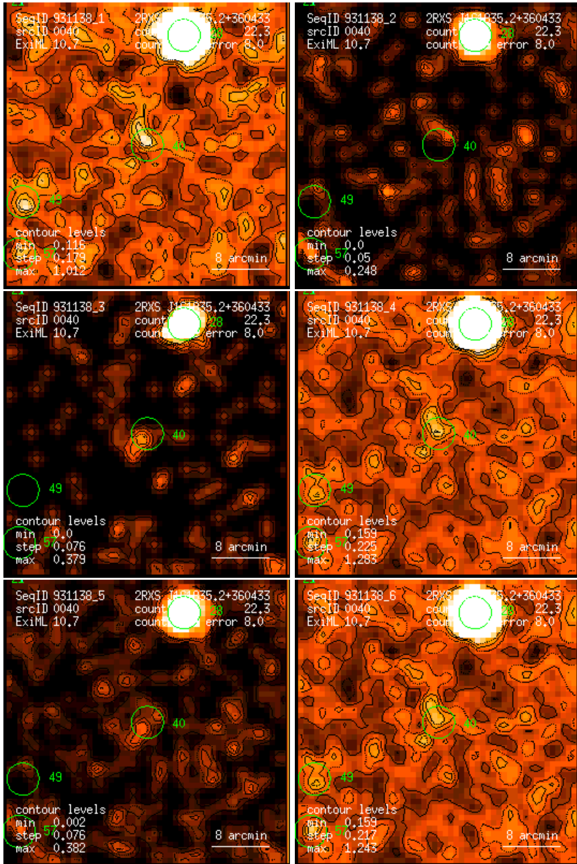
Figure 40: RASS 931138: detection 0040: band rate images, Gaussian filter: (1) PSPC channels 11 – 41, (2) 52 – 90, (3) 91 – 201, (4) 11 – 235, (5) 52 – 201, (6) 11 – 201. Broad band rates in counts/ks. Band rate contour levels in counts/ks/arcmin 2 .
