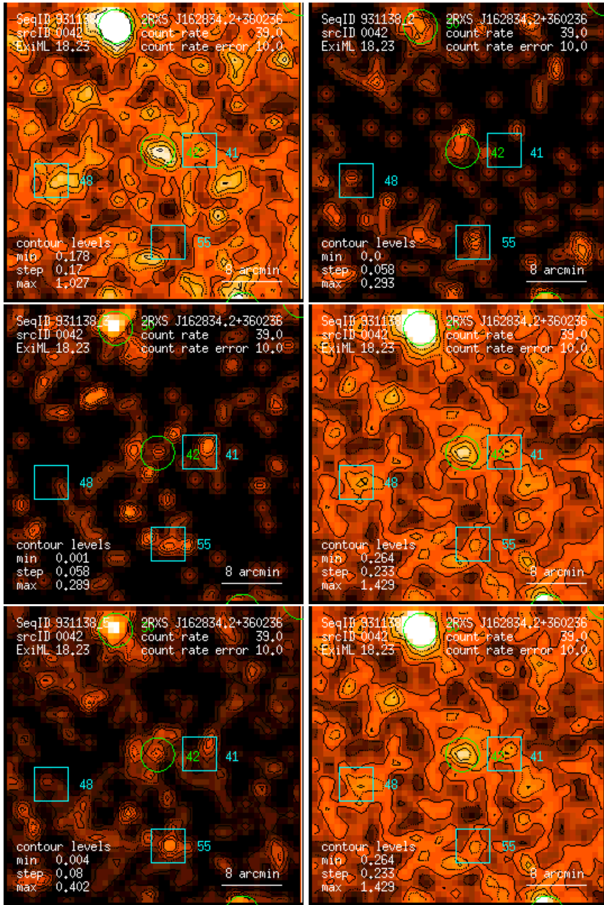
Figure 42: RASS 931138: detection 0042: band rate images, Gaussian filter: (1) PSPC channels 11 – 41, (2) 52 – 90, (3) 91 – 201, (4) 11 – 235, (5) 52 – 201, (6) 11 – 201. Broad band rates in counts/ks. Band rate contour levels in counts/ks/arcmin 2 .
