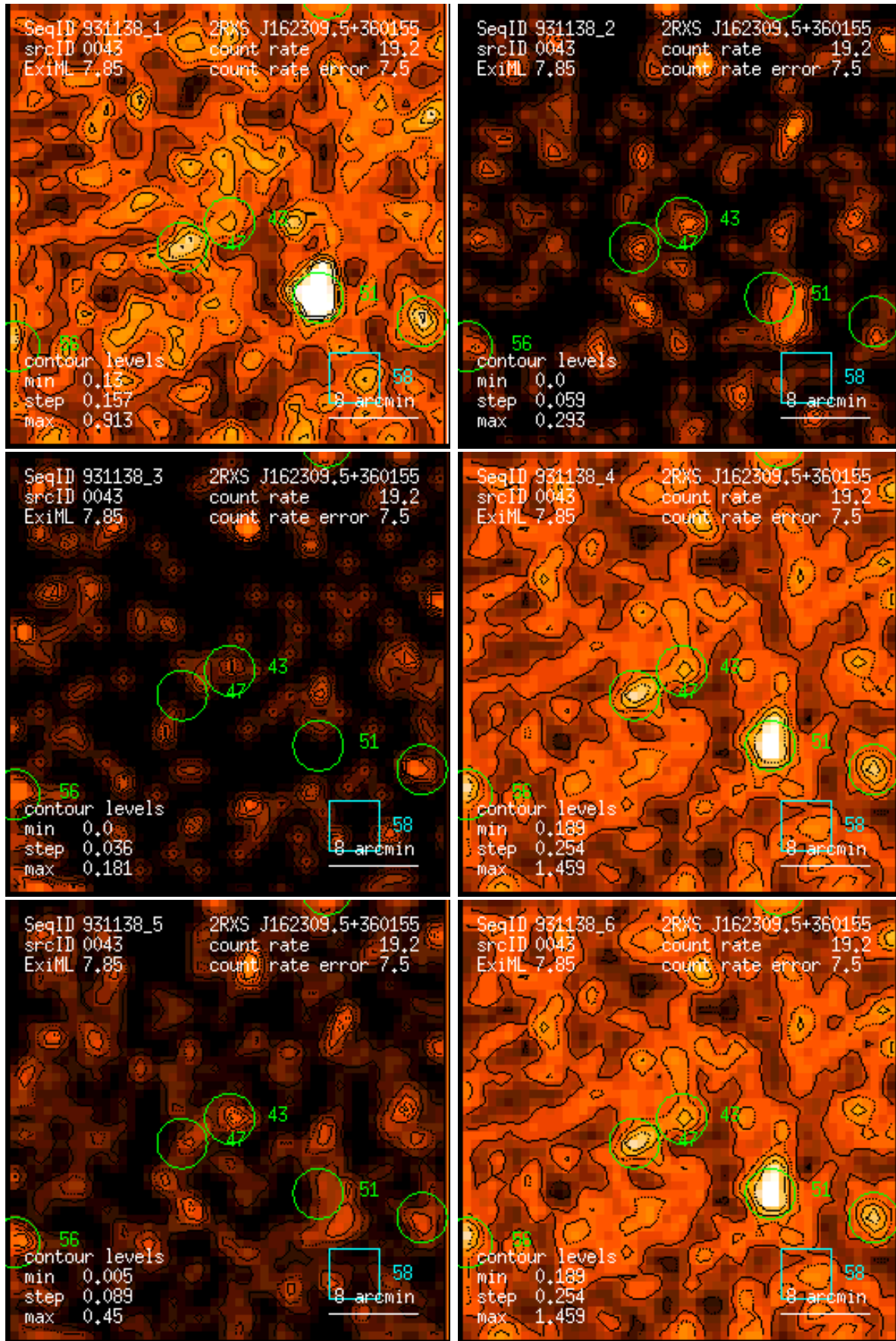
Figure 43: RASS 931138: detection 0043: band rate images, Gaussian filter: (1) PSPC channels 11 – 41, (2) 52 – 90, (3) 91 – 201, (4) 11 – 235, (5) 52 – 201, (6) 11 – 201. Broad band rates in counts/ks. Band rate contour levels in counts/ks/arcmin 2 .
