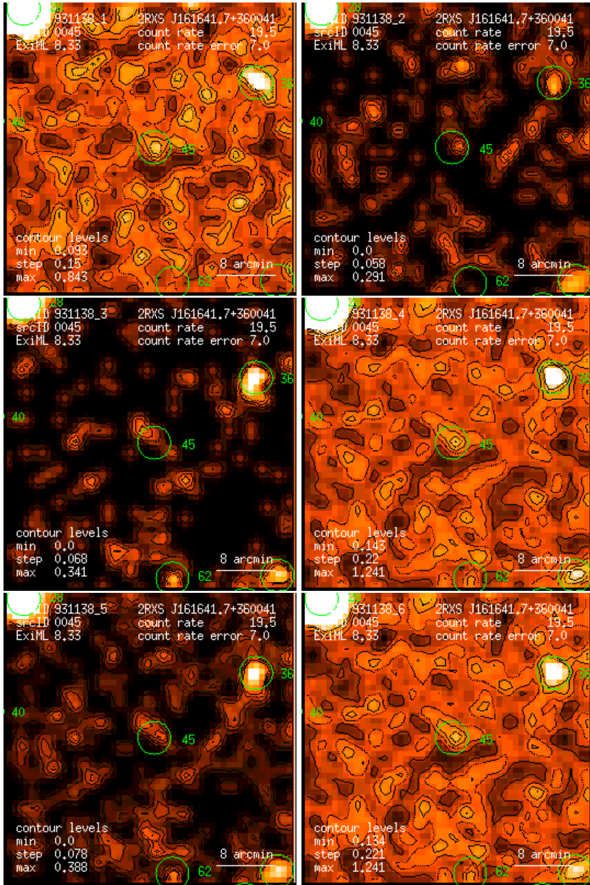
Figure 45: RASS 931138: detection 0045: band rate images, Gaussian filter: (1) PSPC channels 11 – 41, (2) 52 – 90, (3) 91 – 201, (4) 11 – 235, (5) 52 – 201, (6) 11 – 201. Broad band rates in counts/ks. Band rate contour levels in counts/ks/arcmin 2 .
