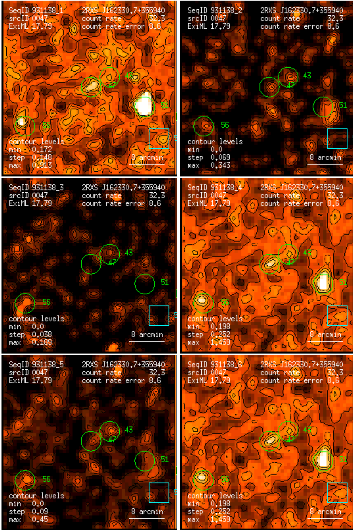
Figure 47: RASS 931138: detection 0047: band rate images, Gaussian filter: (1) PSPC channels 11 – 41, (2) 52 – 90, (3) 91 – 201, (4) 11 – 235, (5) 52 – 201, (6) 11 – 201. Broad band rates in counts/ks. Band rate contour levels in counts/ks/arcmin 2 .
