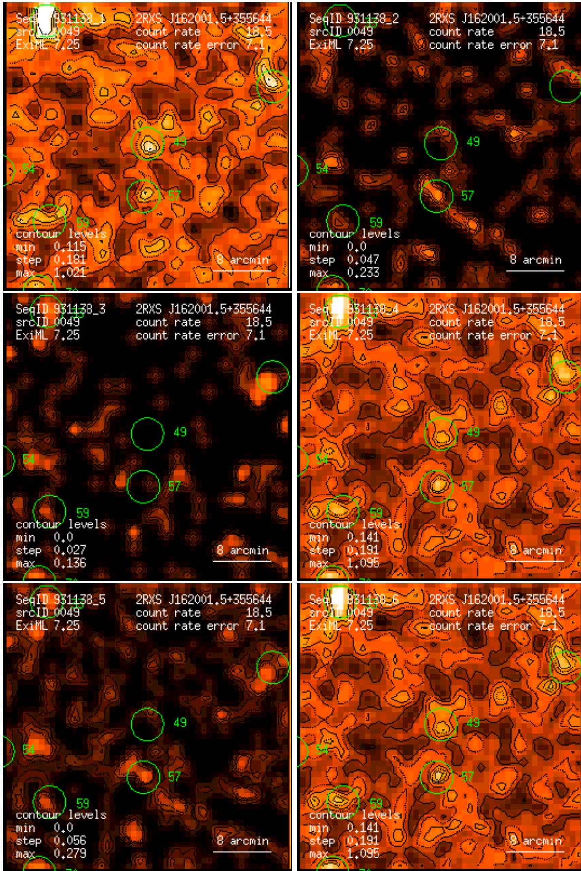
Figure 49: RASS 931138: detection 0049: band rate images, Gaussian filter: (1) PSPC channels 11 – 41, (2) 52 – 90, (3) 91 – 201, (4) 11 – 235, (5) 52 – 201, (6) 11 – 201. Broad band rates in counts/ks. Band rate contour levels in counts/ks/arcmin 2 .
