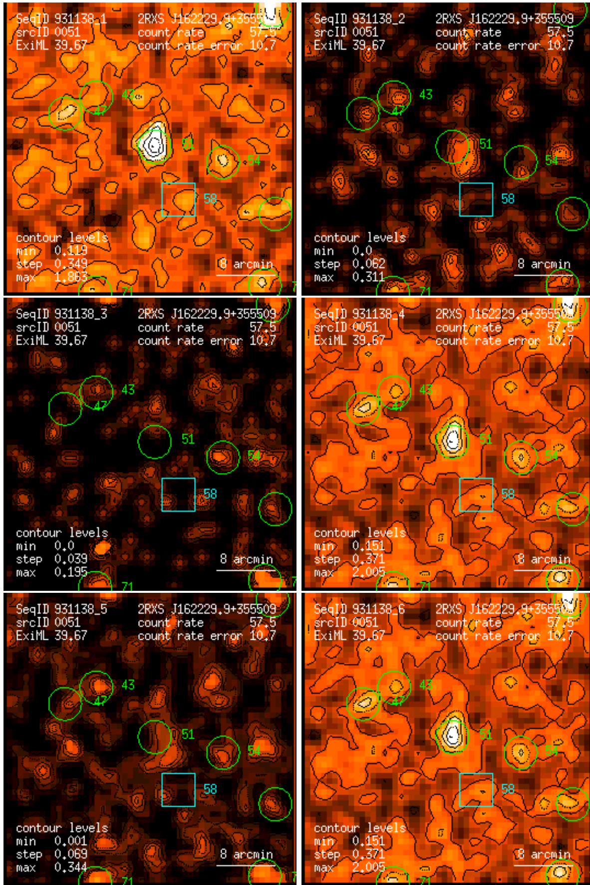
Figure 51: RASS 931138: detection 0051: band rate images, Gaussian filter: (1) PSPC channels 11 – 41, (2) 52 – 90, (3) 91 – 201, (4) 11 – 235, (5) 52 – 201, (6) 11 – 201. Broad band rates in counts/ks. Band rate contour levels in counts/ks/arcmin 2 .
