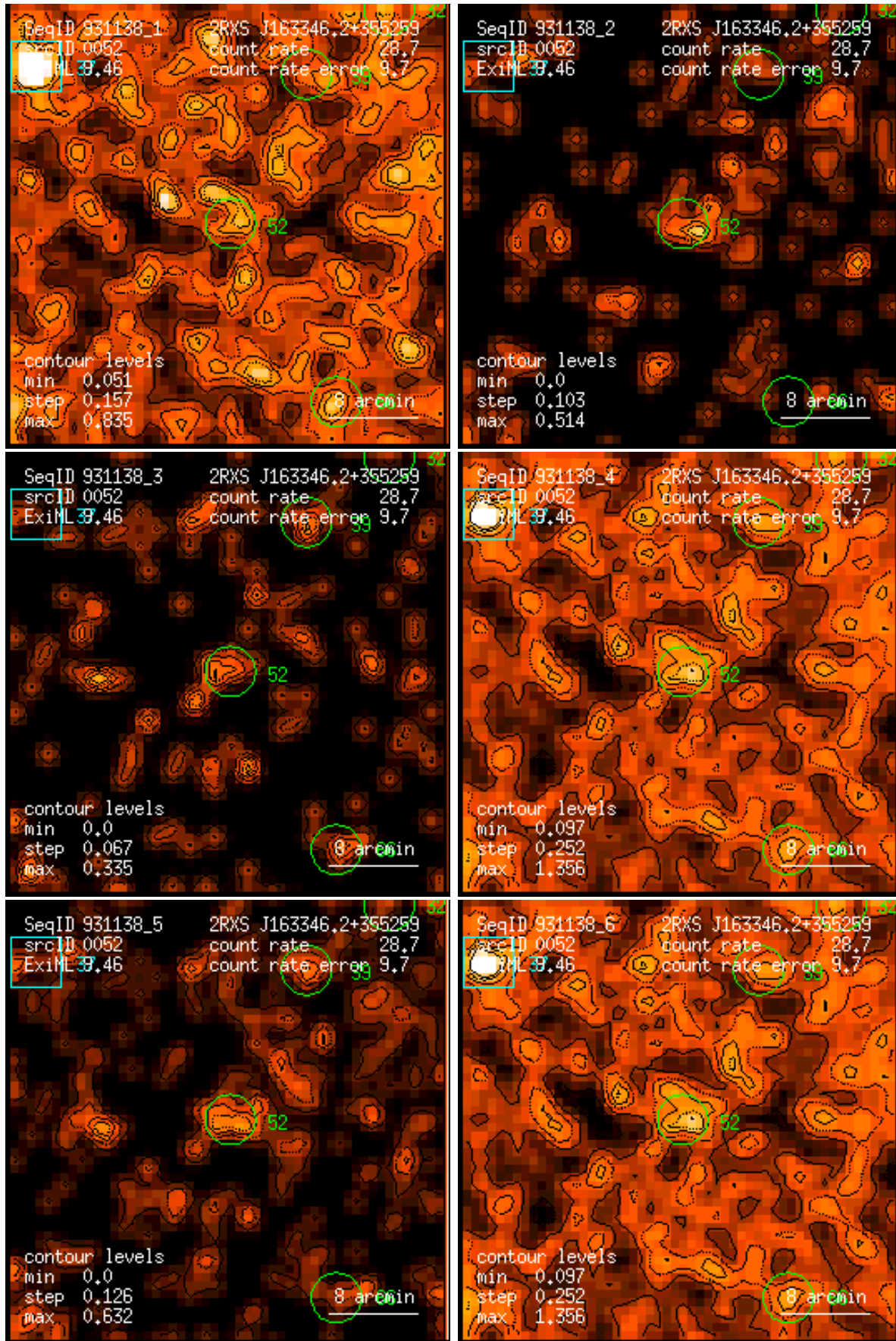
Figure 52: RASS 931138: detection 0052: band rate images, Gaussian filter: (1) PSPC channels 11 – 41, (2) 52 – 90, (3) 91 – 201, (4) 11 – 235, (5) 52 – 201, (6) 11 – 201. Broad band rates in counts/ks. Band rate contour levels in counts/ks/arcmin 2 .
