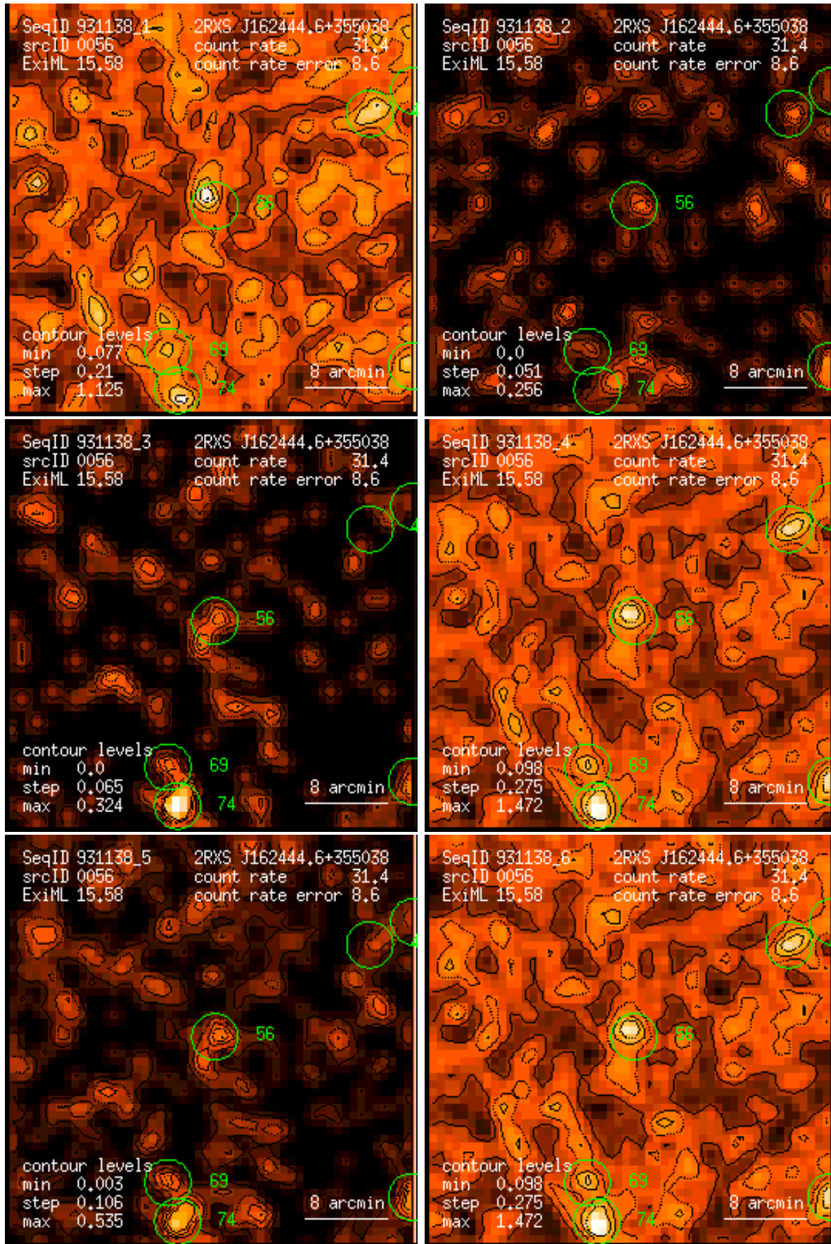
Figure 56: RASS 931138: detection 0056: band rate images, Gaussian filter: (1) PSPC channels 11 – 41, (2) 52 – 90, (3) 91 – 201, (4) 11 – 235, (5) 52 – 201, (6) 11 – 201. Broad band rates in counts/ks. Band rate contour levels in counts/ks/arcmin 2 .
